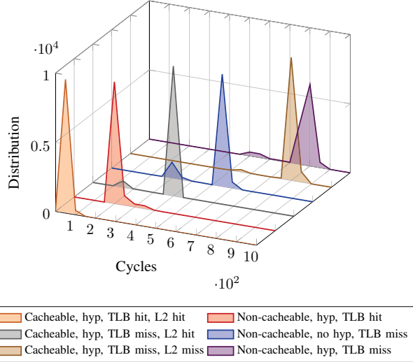
Fig. 5: Distributions of L2 and TLB access time with or without hypervisor.
