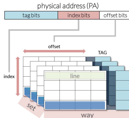
Fig. 1: Structure of a 4-way, 4-sets set-associative cache.
